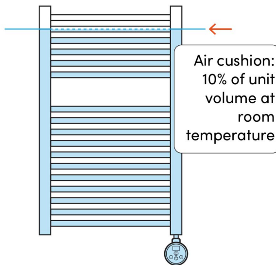
Figure 7 | Air cushion requirement
