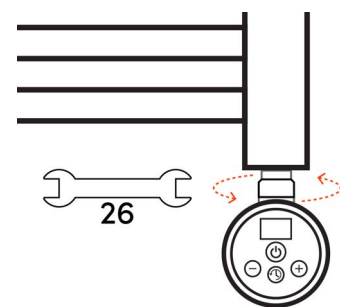
Figure 5 | Tighten element at main nut
